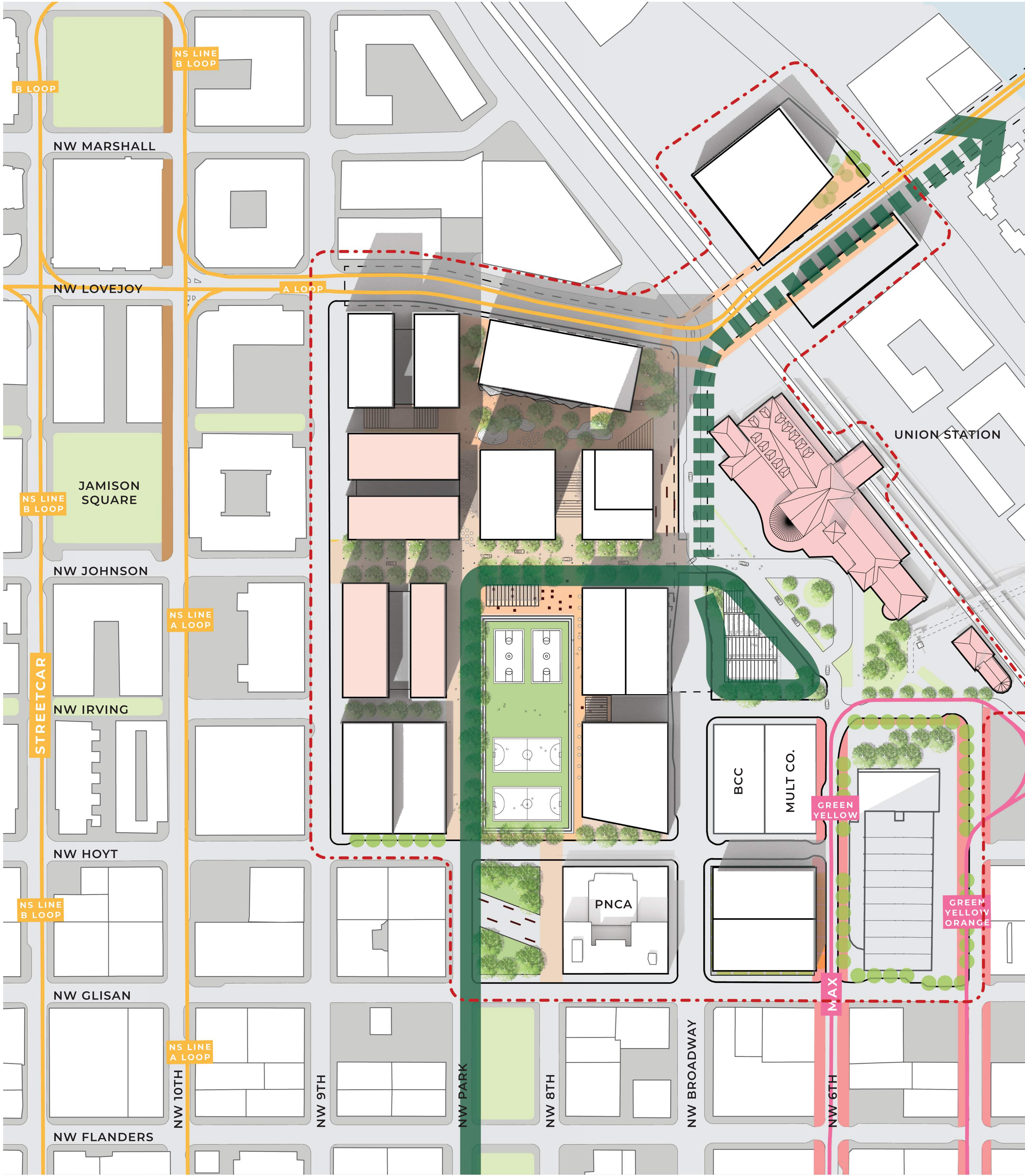
SITE PLAN
